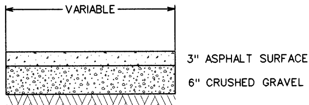
SECTION A-A (NOT TO SCALE)
